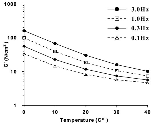
Fig6: Temperature Sensitivities of ISD111 G' ( \delta=50\% )
